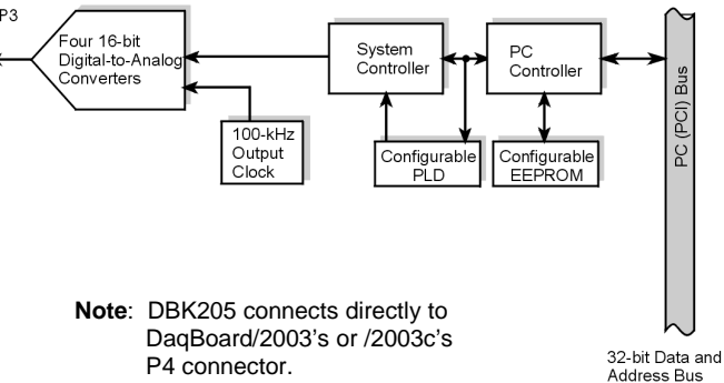
DaqBoard/2003 Block Diagram
